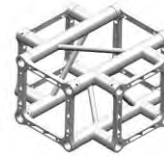
QH40SAX4 HD 40 cm. square 4 way cross
