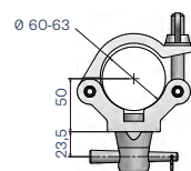
LT C370 Truss clamp ALI6063 1/2 spigot swl 500kg
