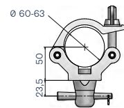
LT C370 Truss clamp AL16063 1/2 spigot swl 500kg
