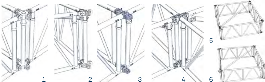
1 / FL76 truss fixed onto 4-way connection system FL76CS04
