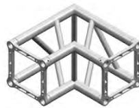
QH40SAL2090 HD 40 cm. square 2 way 90° corner
