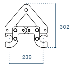
QU3040H050 30-40 Special Truss L=050 with hoist support
