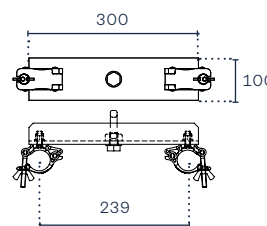
CBT3040 2 points Bridle Hook for 29/40 cm. truss
