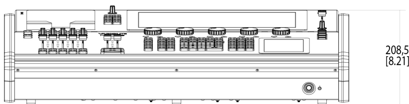
Figure 2: Neo X5 Dimensioned drawings
